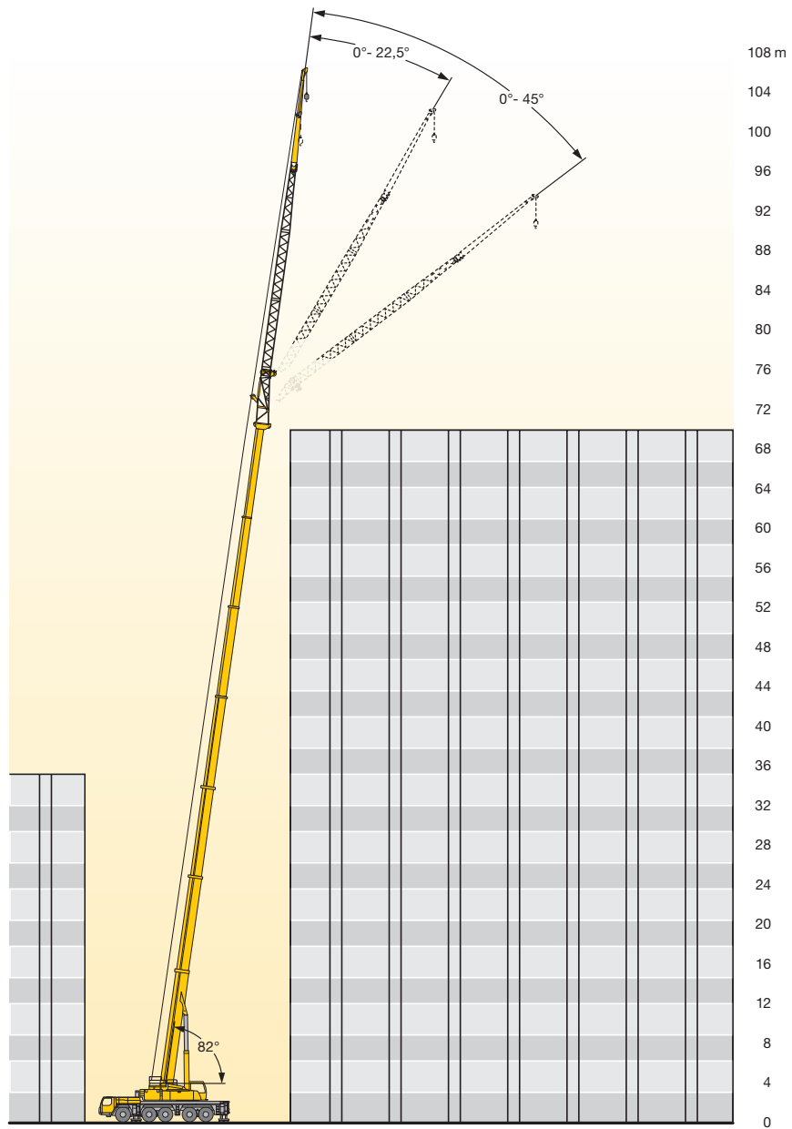
Adjustable folding jib (0° to 45°)
