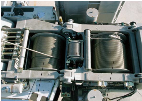
Winch 1 Auxiliary winch Winch 2 Winch 3
