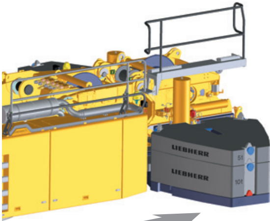
Partial counterweight, radius 5.6 m
