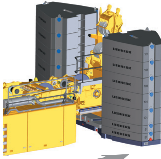
140 t total counterweight, radius 6.6 m
